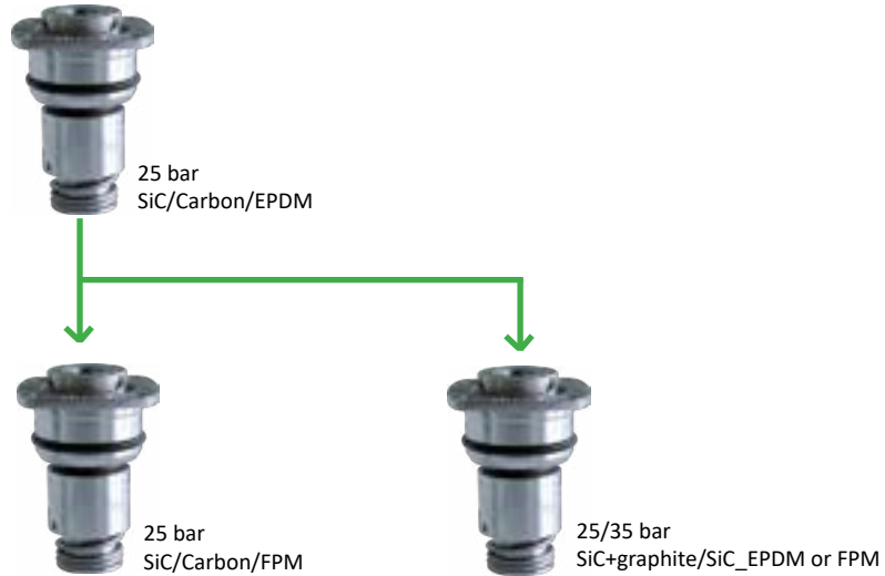
Balanced cartridge type
